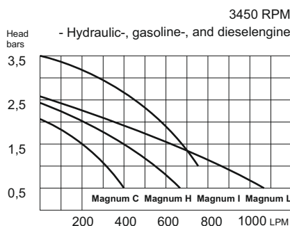
Magnum with diesel engine and Roll Cage
